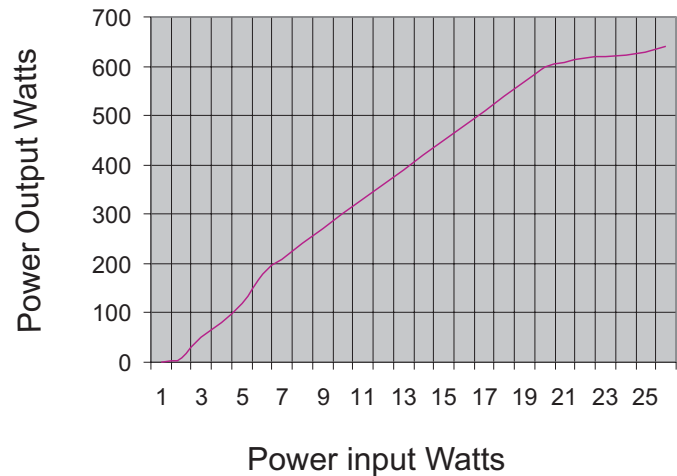
Power Output V Power input at 45V
