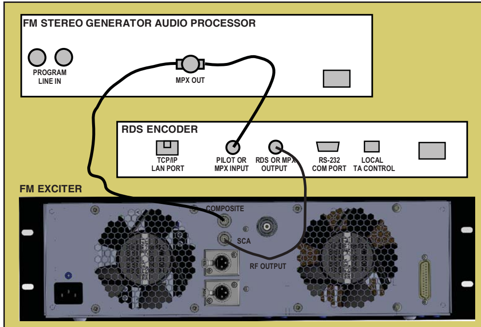
Sidechain Encoder Connection
