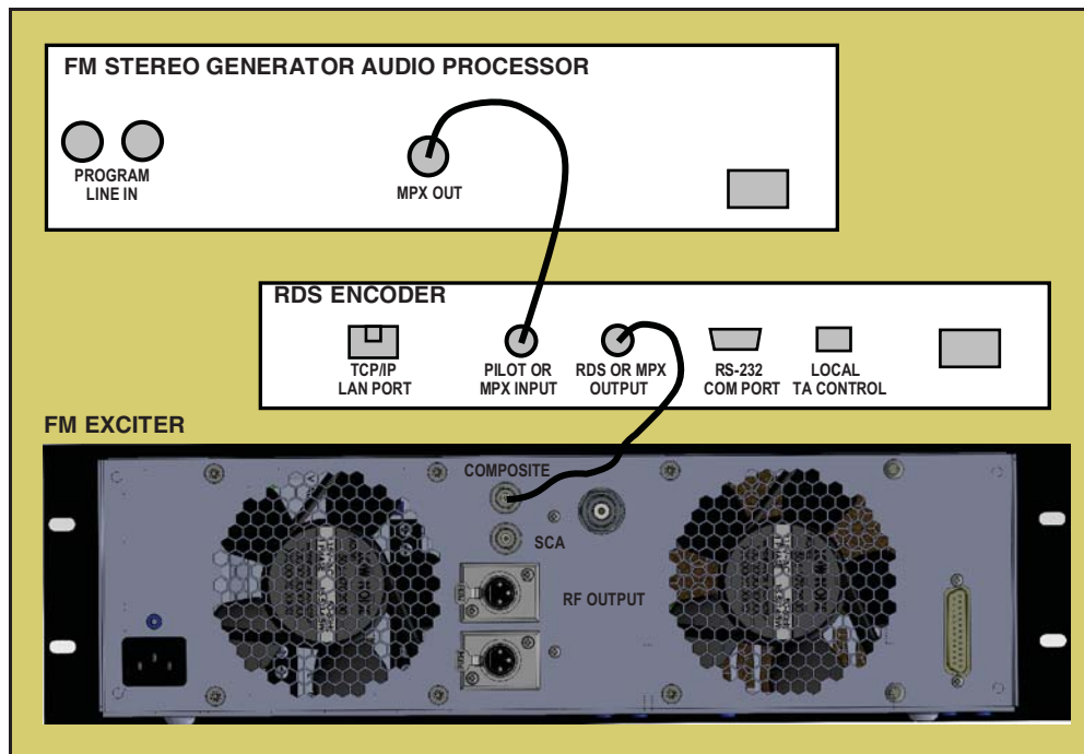
Loop-Through Encoder Connection
